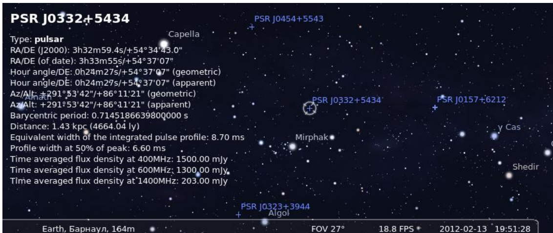
Figure 13.5: PSR J0332-5434
