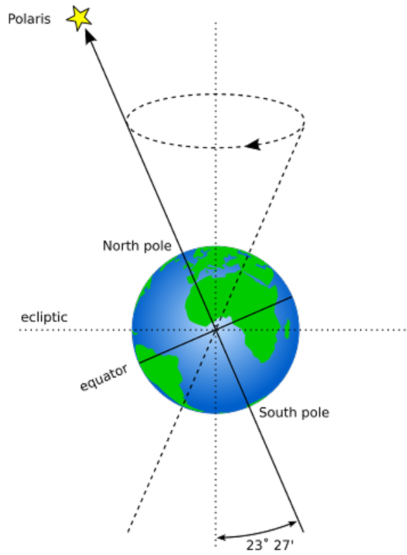
Figure 17.5: Precession
