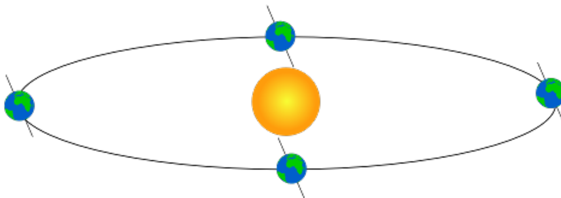
Figure 17.4: Ecliptic obliquity
