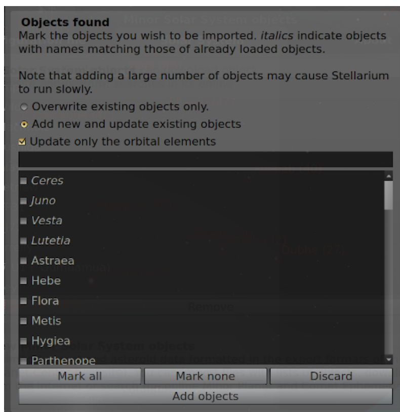
Figure 13.9: Interface of Solar System Editor plugin: Import data dialog — view after downloading and parsing the MPC data.
