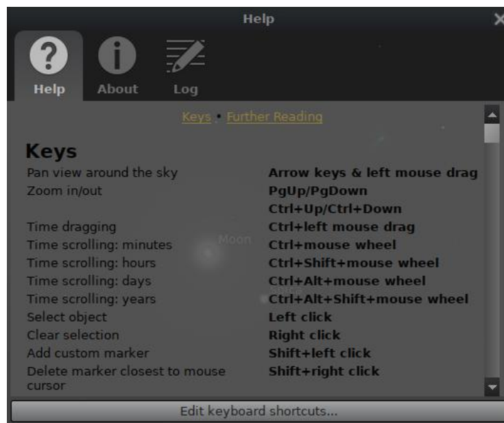
Figure 4.44: Help Window
