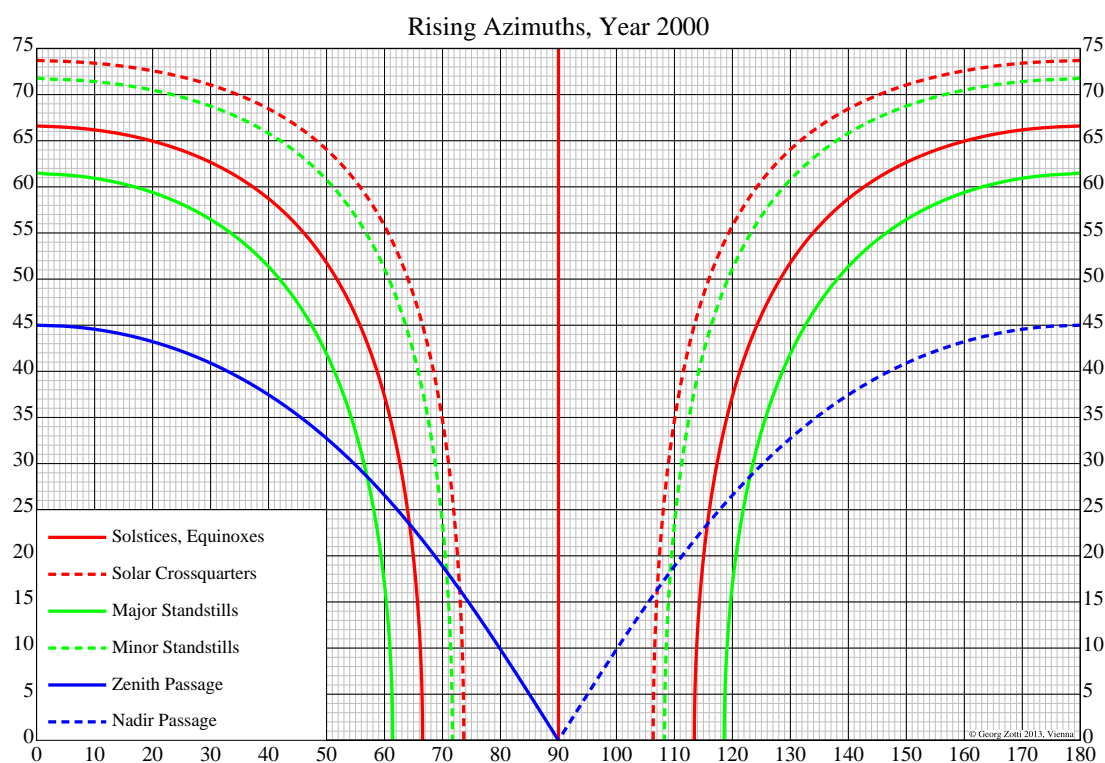
Figure 14.13: Rising azimuths of a few important events for sun and moon, and zenith and nadir passages depending on geographic latitudes (vertical axis).
