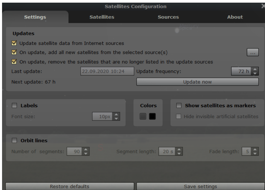
Figure 14.9: Configuration of the Satellites plugin.
