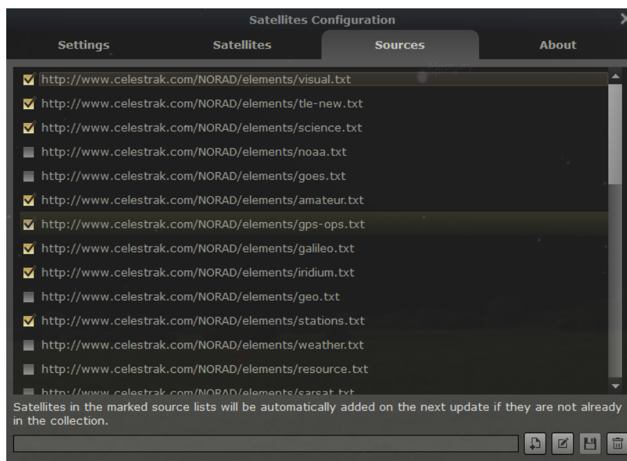
Figure 14.11: Configuration of the Satellites plugin — sources for TLE data.
