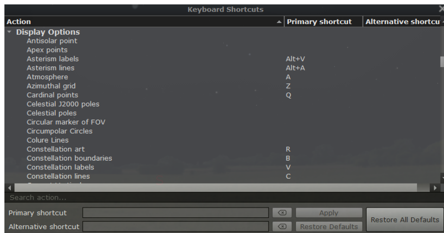
Figure 4.47: Keyboard Shortcuts
