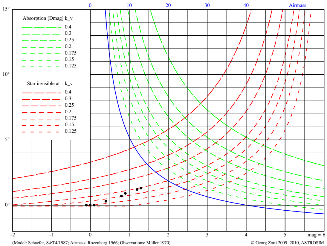
Figure 19.5: Airmass and Extinction. The figure shows Airmass (blue) along the line of sight in the altitude labeled on the left side. The green curves show how many magnitudes an object is dimmed down, depending on extinction factor k (called k_v in the figure). The red curves indicate at which altitude a star of given magnitude can be seen with good eyesight, again depending on k . The black dots are observed values found in the literature.
